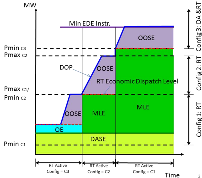
Exhibit C-32: Real-Time Economic Dispatch Levels with Incremental Exceptional Dispatch Instruction
