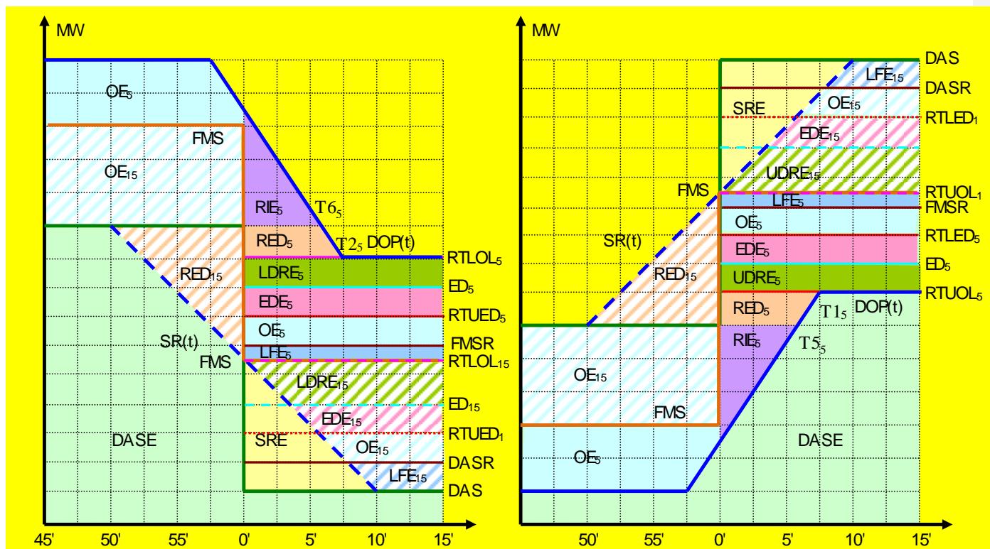
Figure 5a. Instructed imbalance Energy Stack – generation side
