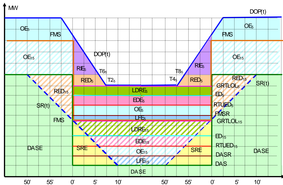
Figure 5f Instructed Imbalance Energy Stack for a NGR. Generation side, RTD dispatch greater than DA schedule.
