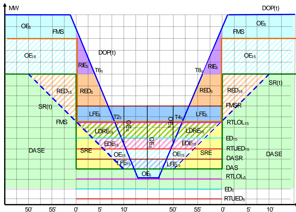
Figure 5r Instructed Imbalance Energy Stack for Generating Resource. Special DRE & EDE Case. At various intervals RTD dispatch is either greater than or less than DA schedule.
