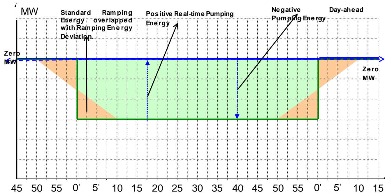
Exhibit C-12: Positive Real-time Pumping Energy
